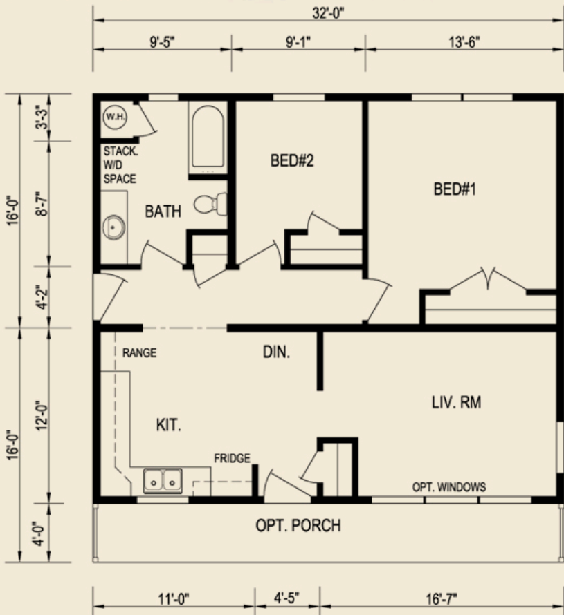
Plan 9107, 32' X 28', 896 sq. ft.
