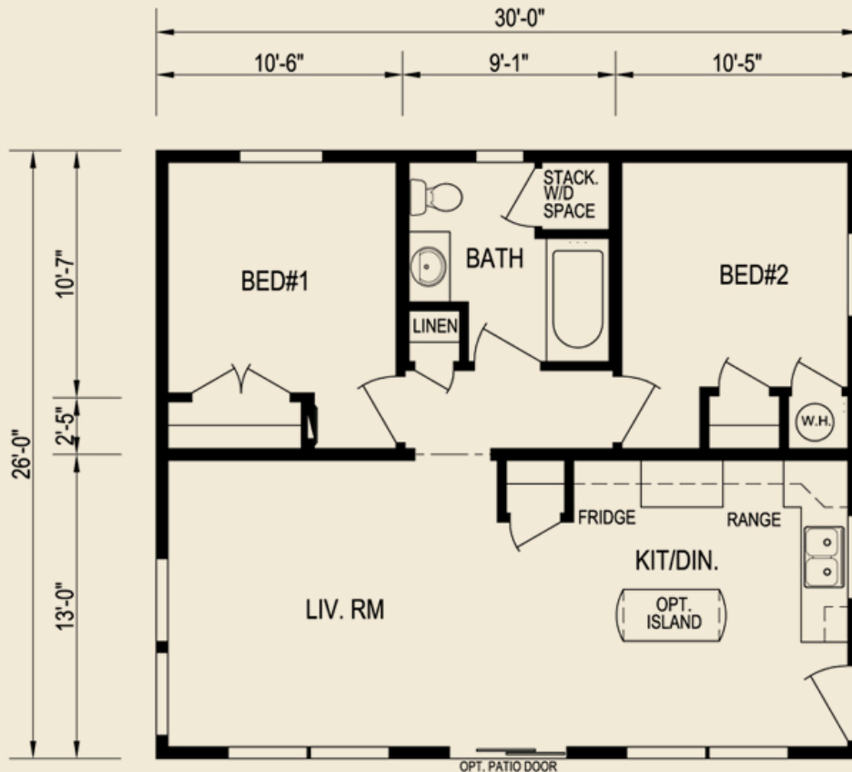
Plan 9106, 30' X 26', 780 sq. ft.
