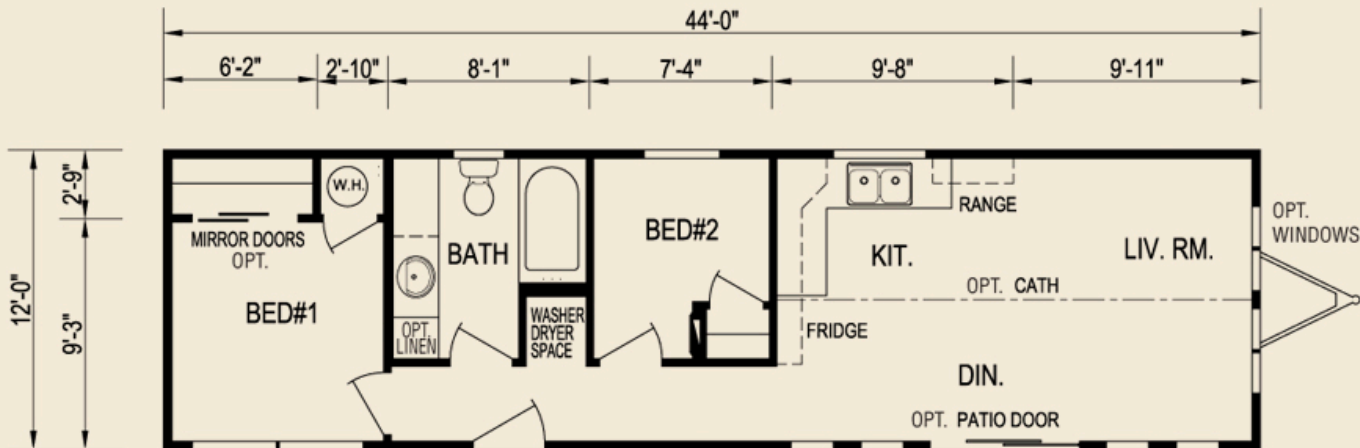
Plan 9103, 44' X 12', 528 sq. ft.
