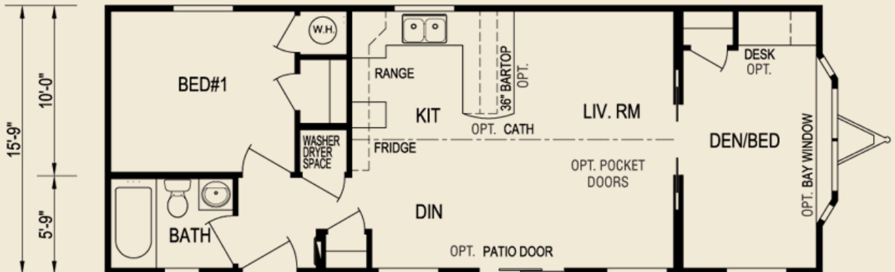
Plan 9102, 42' X 15'-9", 662 sq. ft.
