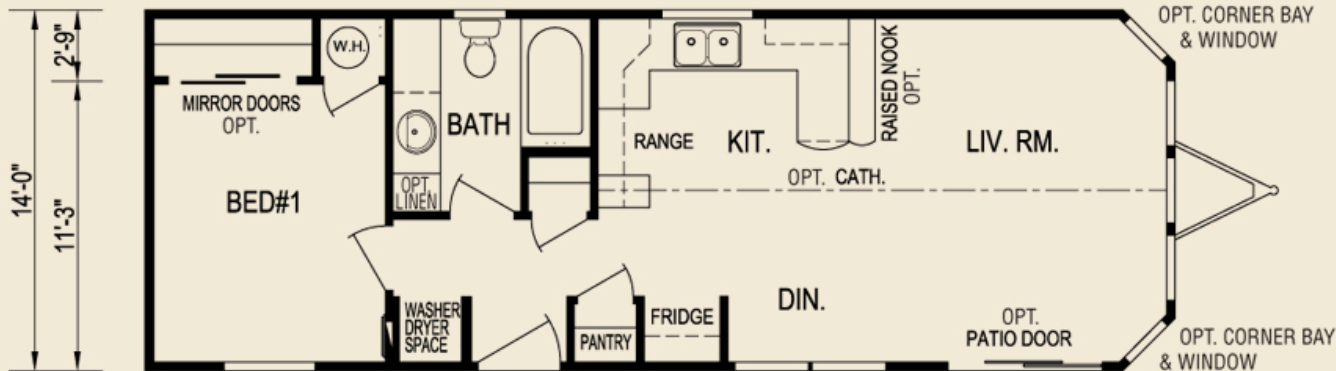
Plan 9101, 40' X 14', 560 sq. ft.
