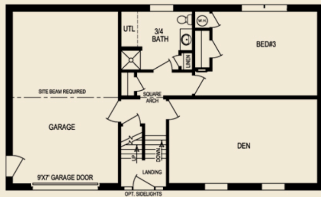
Proposed Basement Layout (on site by others)
