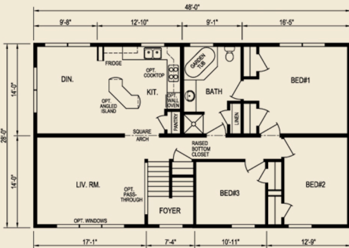
First Floor 1344 sq. ft.
