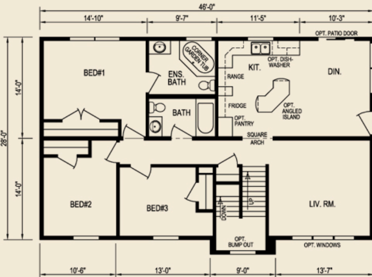
First Floor 1248 sq. ft.
