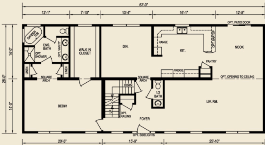
First Floor 1736 sq. ft.
