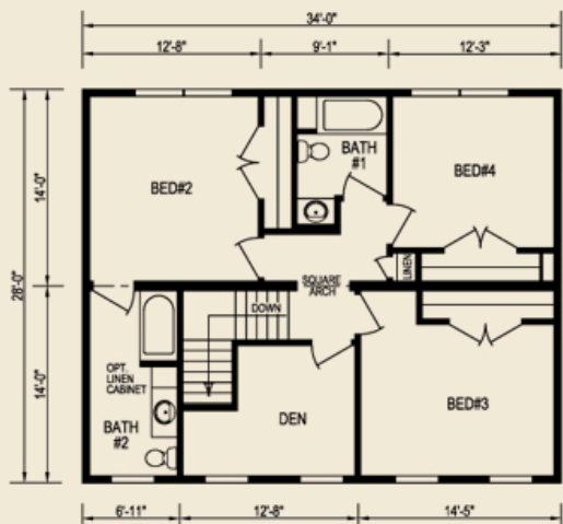
Second Floor 34' X 28', 952 sq. ft.
