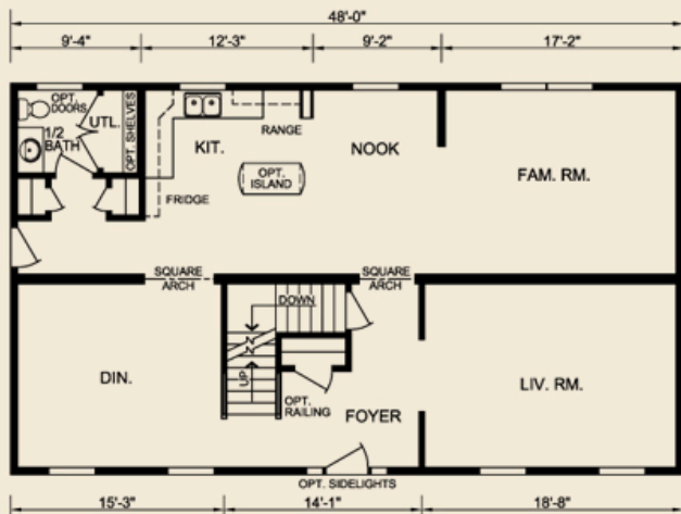
First Floor 1344 sq. ft.
