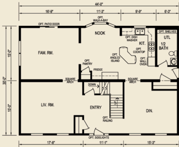
First Floor 1320 sq. ft.
