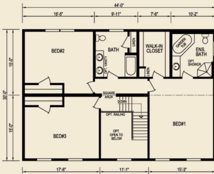
Second Floor 1320 sq. ft.
