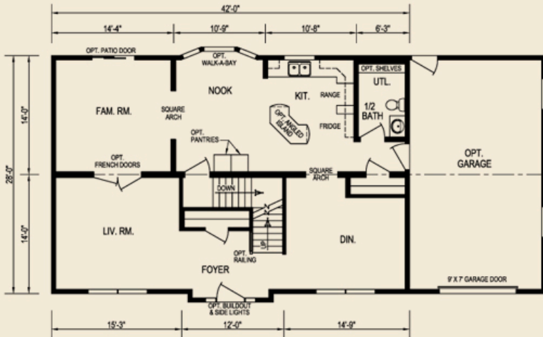
First Floor 1176 sq. ft.
