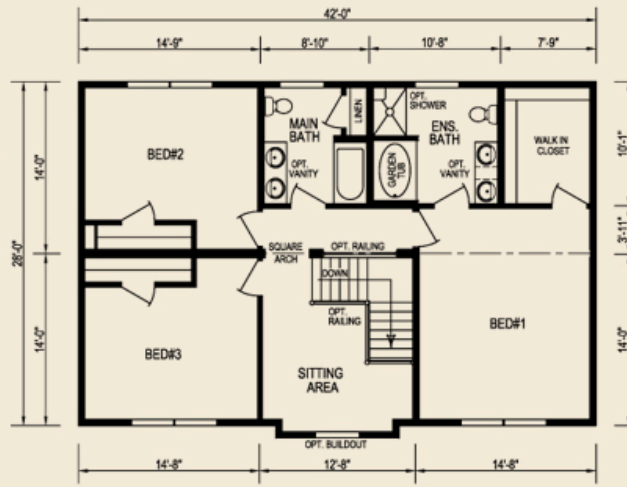
Second Floor 1176 sq. ft.
