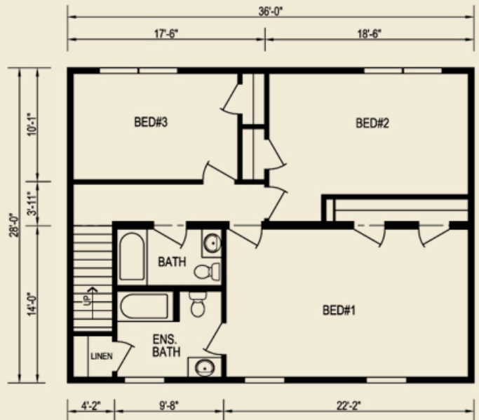
Second Floor 1008 sq. ft.
