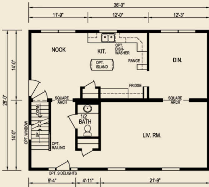
First Floor 1008 sq. ft.
