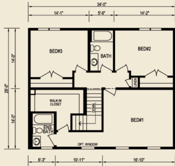
Second Floor 952 sq. ft.
