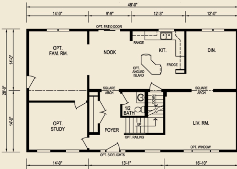
First Floor 952 sq. ft.
