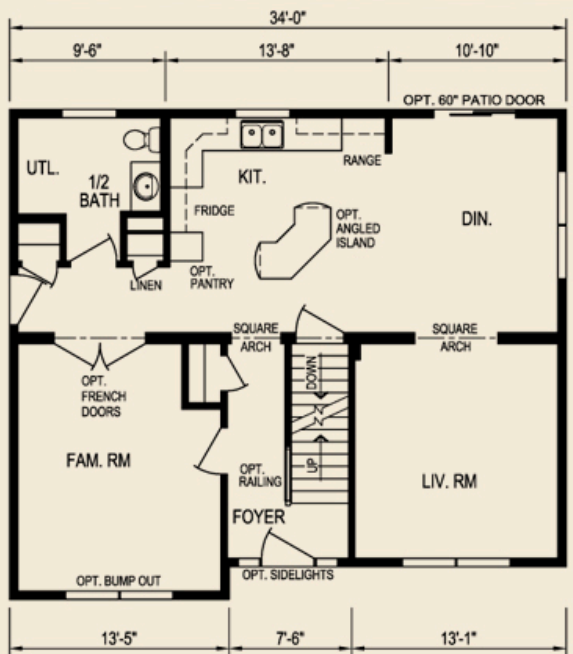
First Floor 952 sq. ft.
