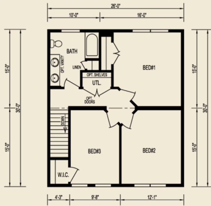
Second Floor 780 sq. ft.
