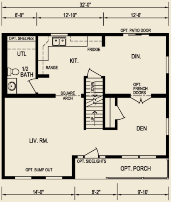
First Floor 768 sq. ft.
