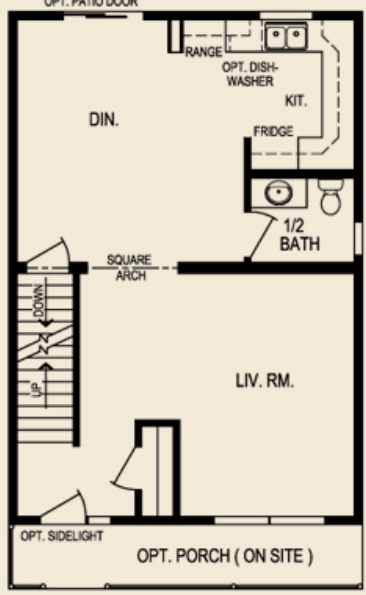
First Floor 704 sq. ft.
