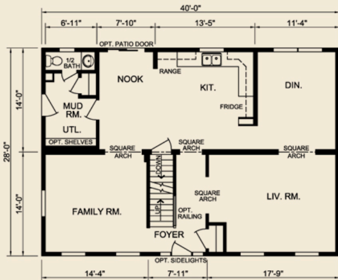
First Floor 1120 sq. ft.
