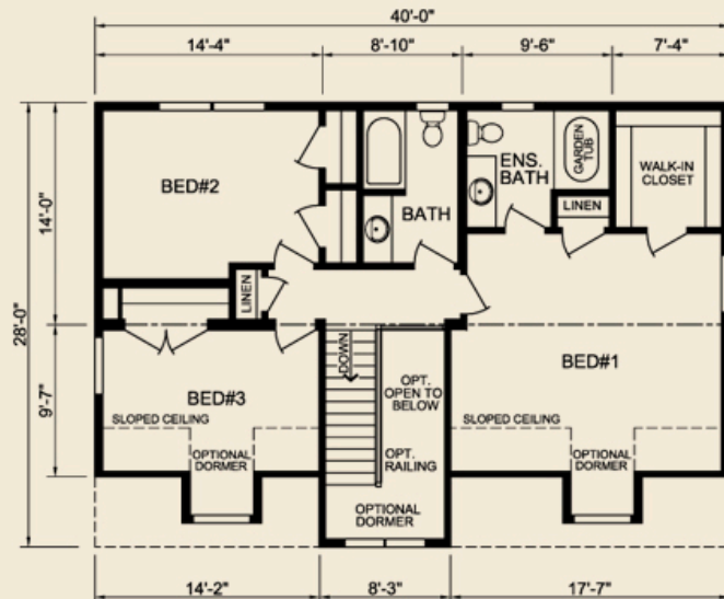
Second Floor 1009 sq. ft.
