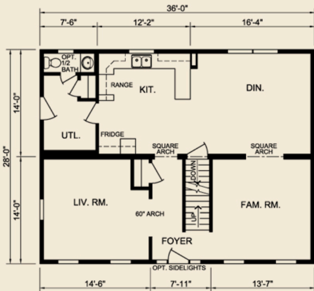
First Floor 1008 sq. ft.
