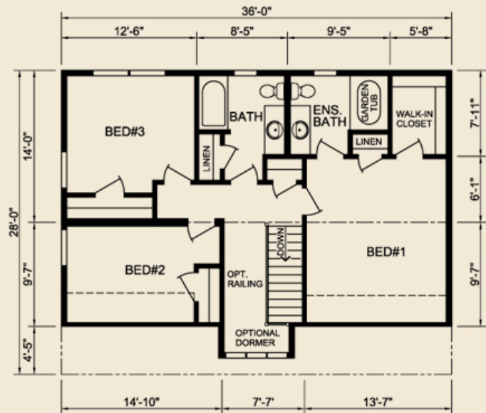
Second Floor 850 sq. ft.
