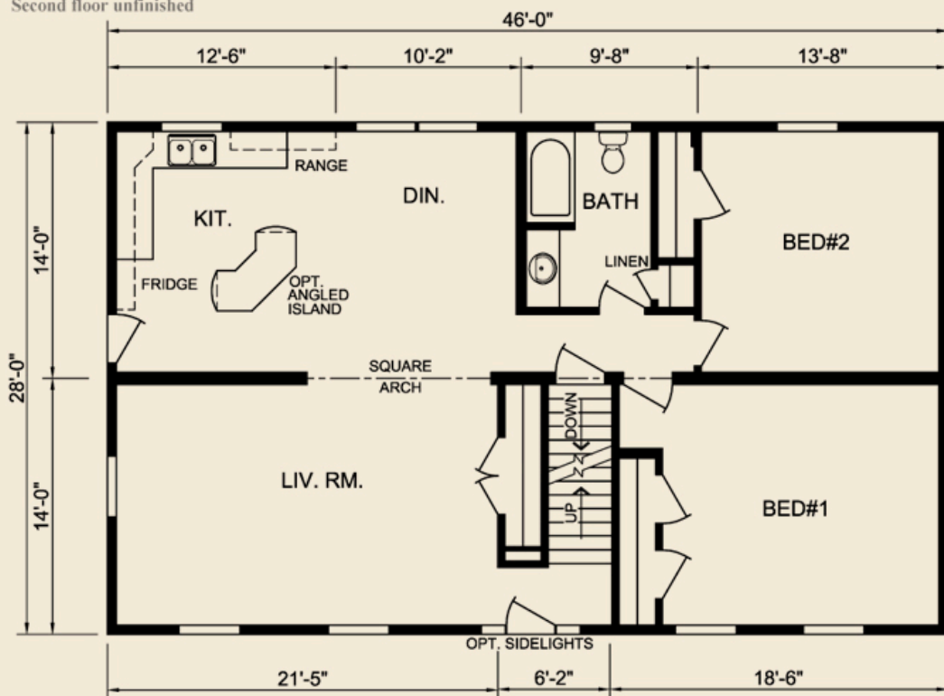
Plan 8305, 46' X 28', 1288 sq. ft.
