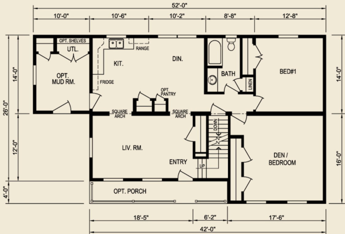
Plan 8304, 42' X 30'/26', 1162 sq. ft.
