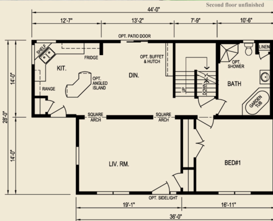
Plan 8302, 44'/36' X 28', 1120 sq. ft.
