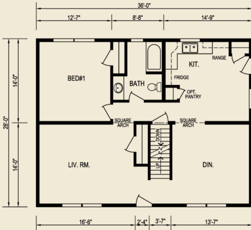
Plan 8301, 36' X 28', 1008 sq. ft.
