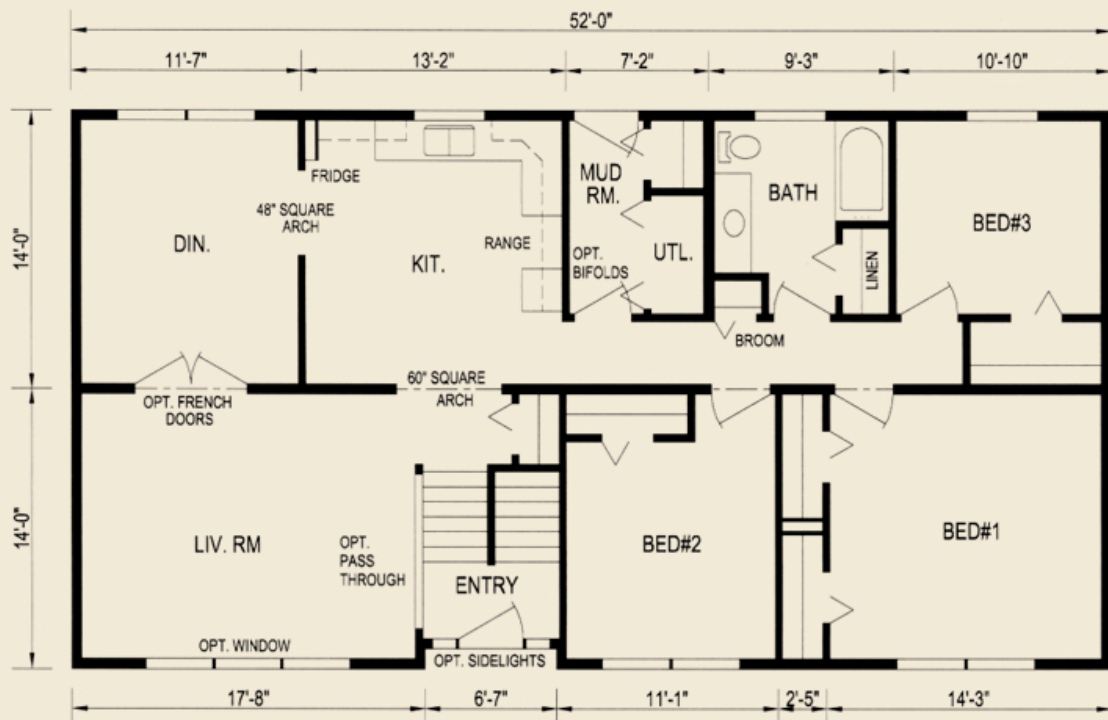
Plan 7231, 52' X 28', 1456 sq. ft.
