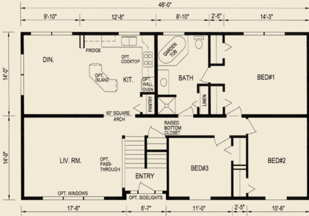
Plan 7230, 48' X 28', 1344 sq. ft.
