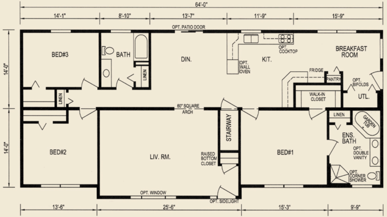
Plan 7225, 64' X 28', 1792 sq. ft.
