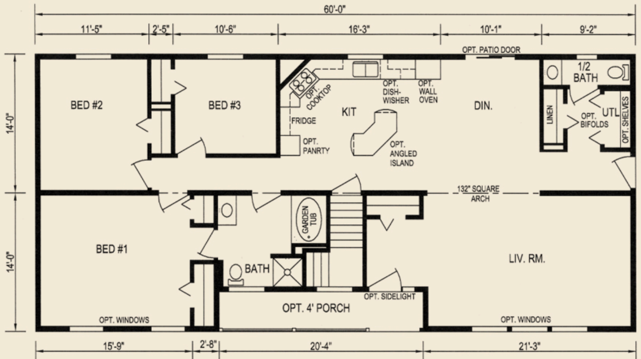
Plan 7223, 60' X 28'24", 1599 sq. ft.
