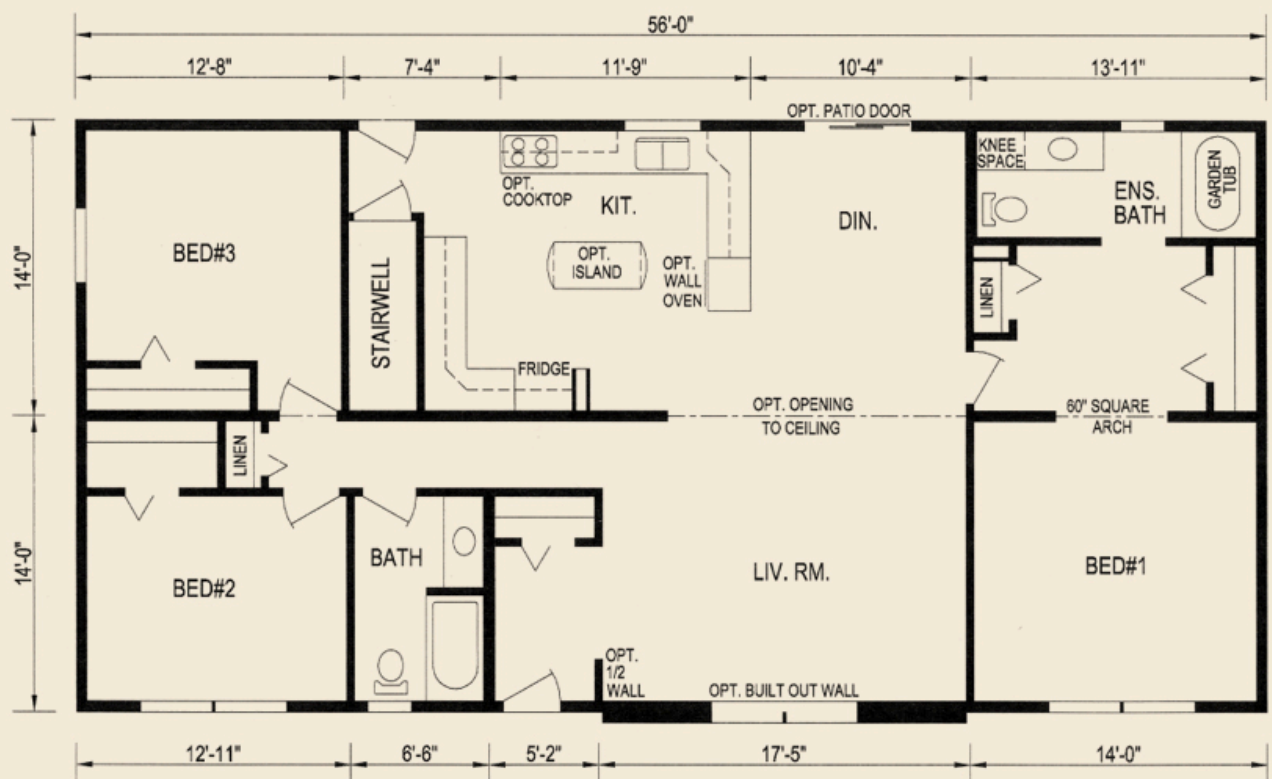
Plan 7222, 56' X 28', 1568 sq. ft.
