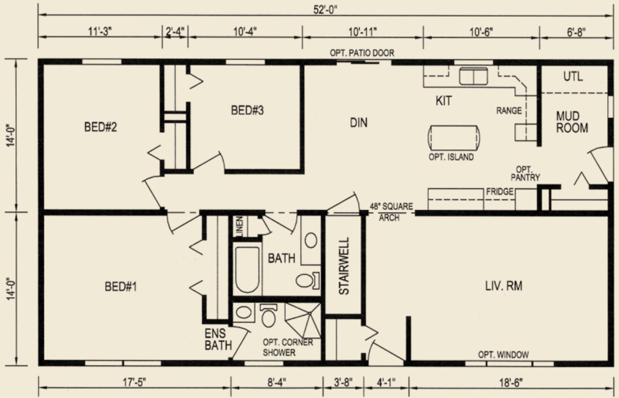
Plan 7221, 52' X 28', 1456 sq. ft.
