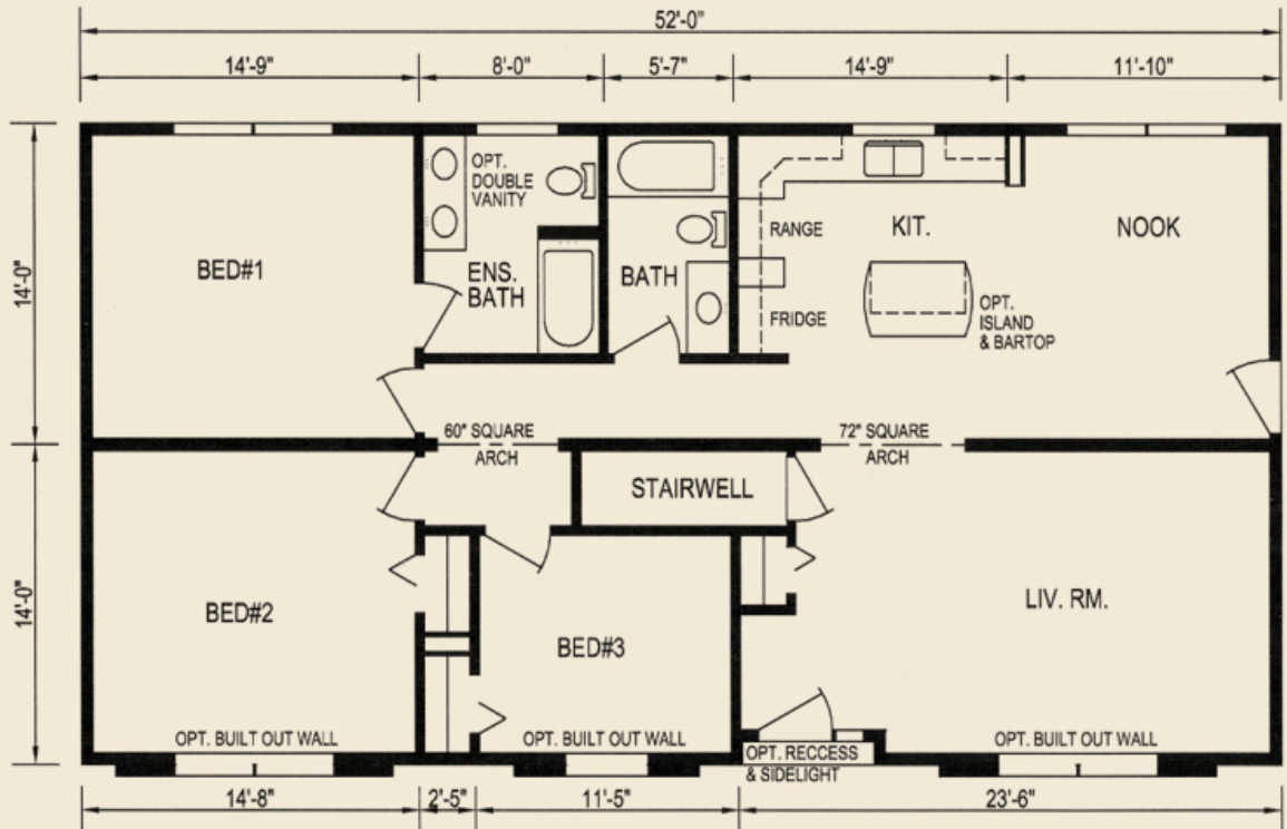
Plan 7219, 52' X 28', 1456 sq. ft.
