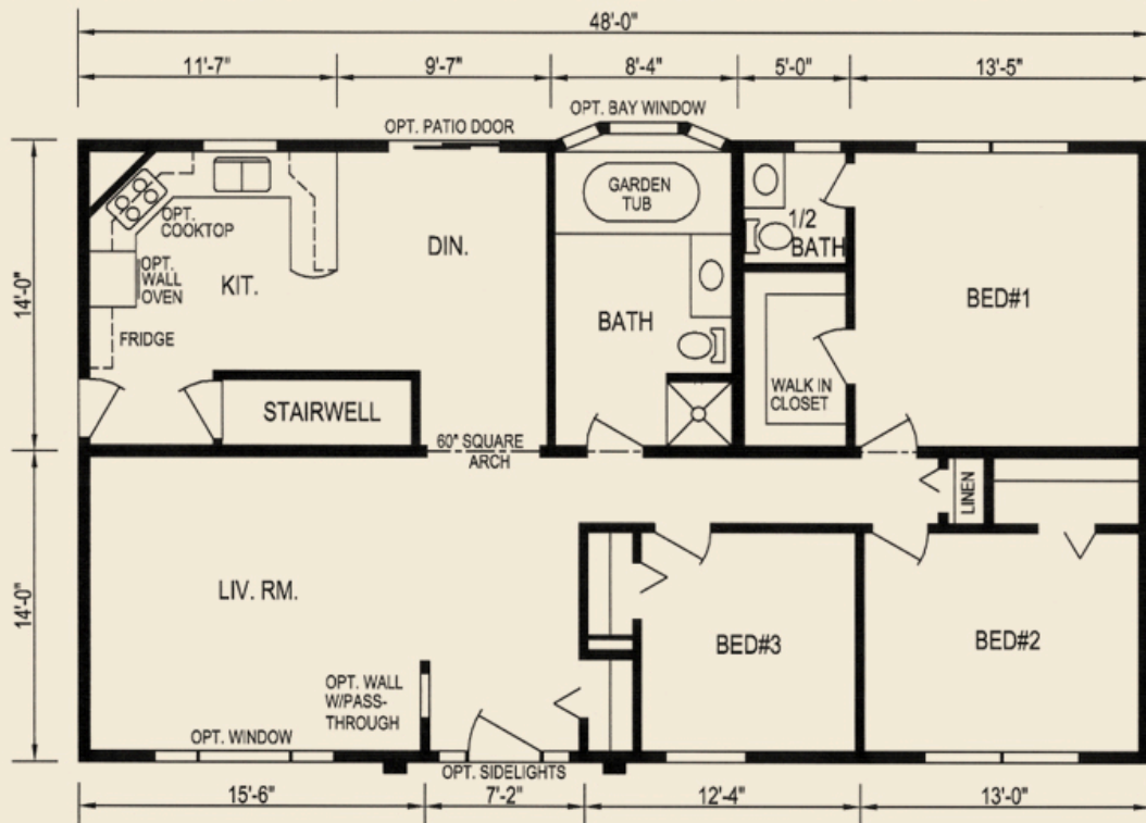
Plan 7218, 48' X 28', 1344 sq. ft.
