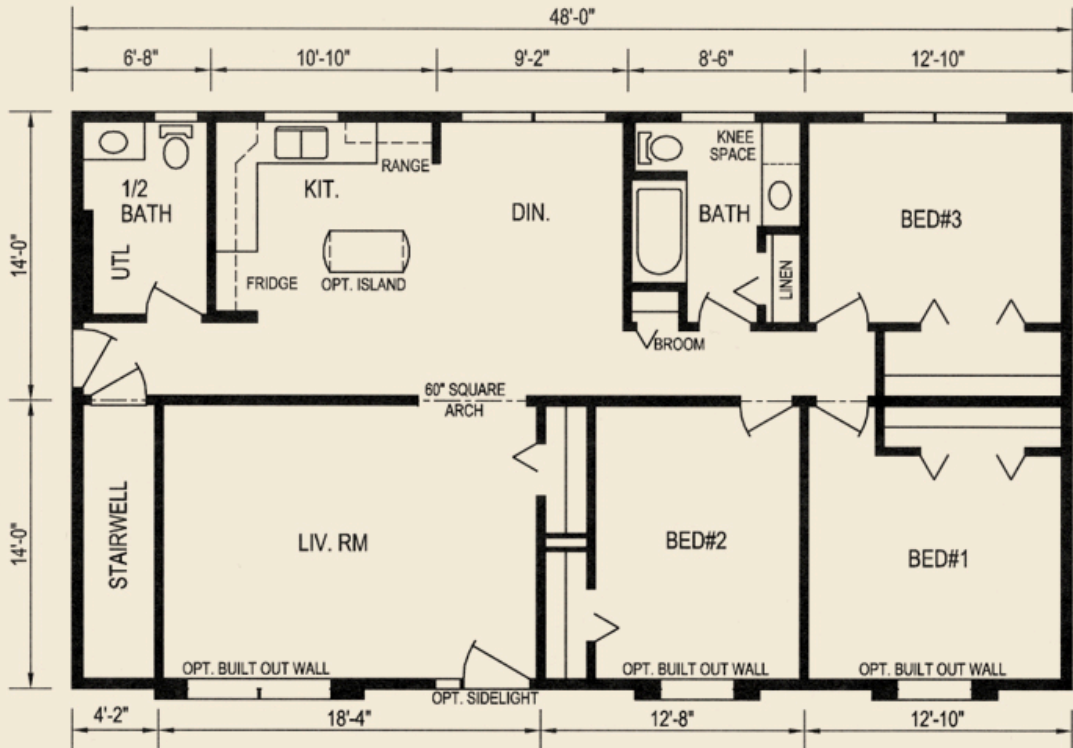
Plan 7217, 48' X 28', 1344 sq. ft.
