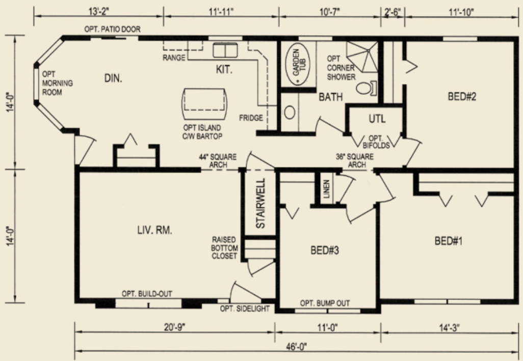
Plan 7213, 46 X 28', 1288 sq. ft.
