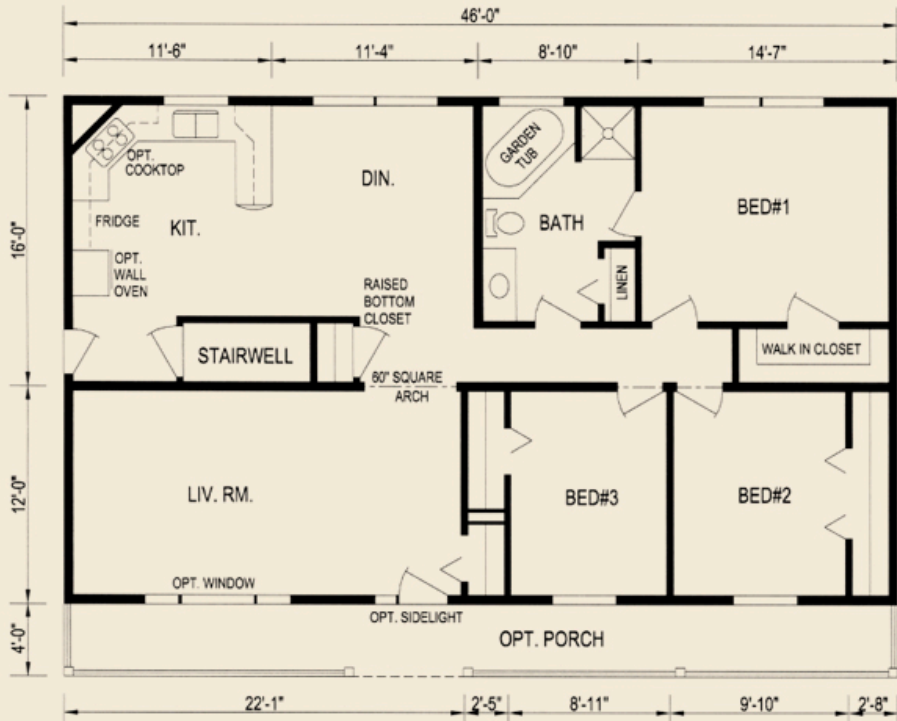
Plan 7212, 46' X 28', 1288 sq. ft.
