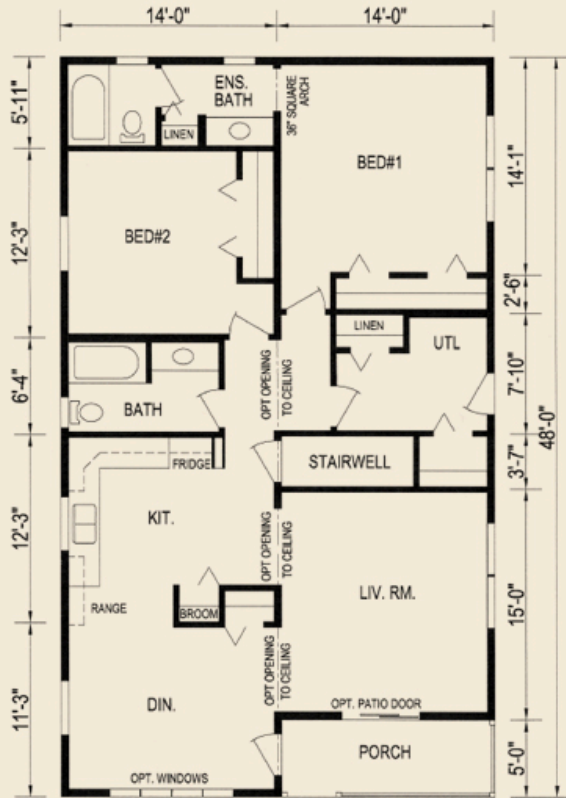
Plan 7210, 48'/43' X 28', 1274 sq. ft.
