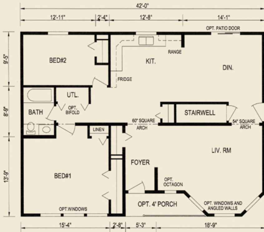
Plan 7209, 42' X 32', 1244 sq. ft.
