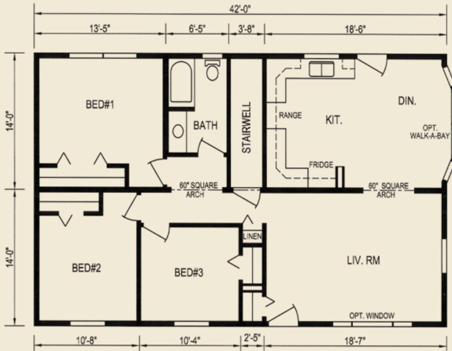
Plan 7206, 42' X 28', 1176 sq. ft.
