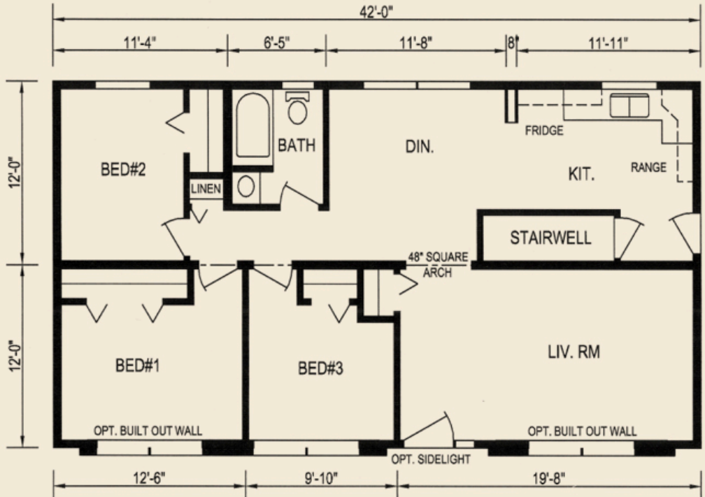
Plan 7203, 42' X 24', 1008 sq. ft.
